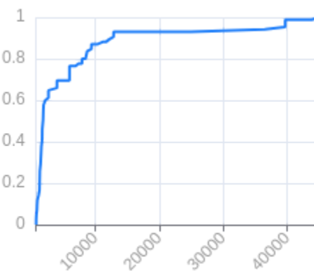
Summary stats
